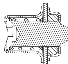
Fig. 30 Sectional drawing of deblocking device
