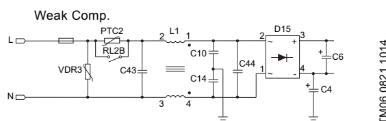
Fig. 43 Relay and PTC
