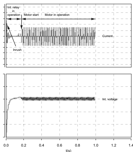
Fig. 44 Example: UPM3 with internal inrush relay
