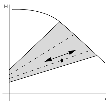
Fig. 23 New lower proportional pressure curve
