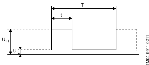
Fig. 4 PWM signal
