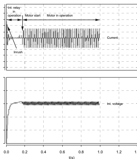
Fig. 44 Example: UPM3 with internal inrush relay
